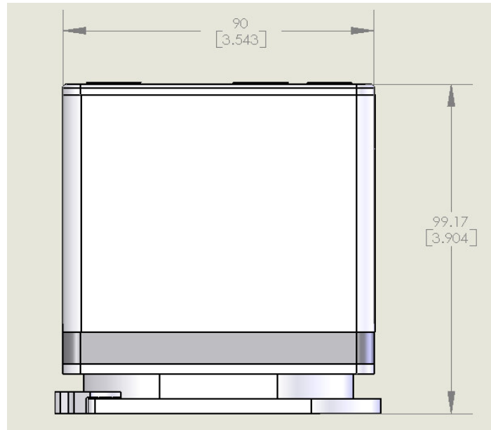
Figure 3: Enclosed Body (Type D) with Split Flange (Type C) - Top View
