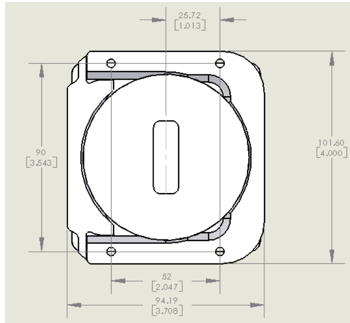
Figure 1: Enclosed Body (Type D) with Split Flange (Type C) – Front View
