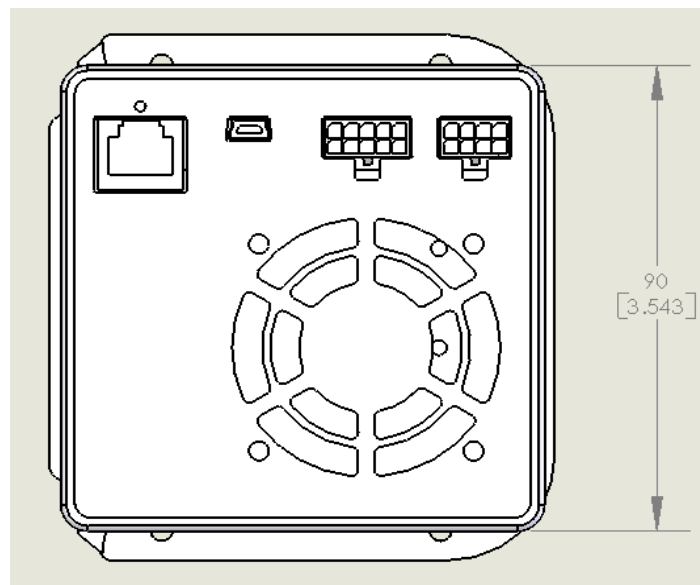
Figure 2: Enclosed Body (Type D) with Split Flange (Type C) - Back View
