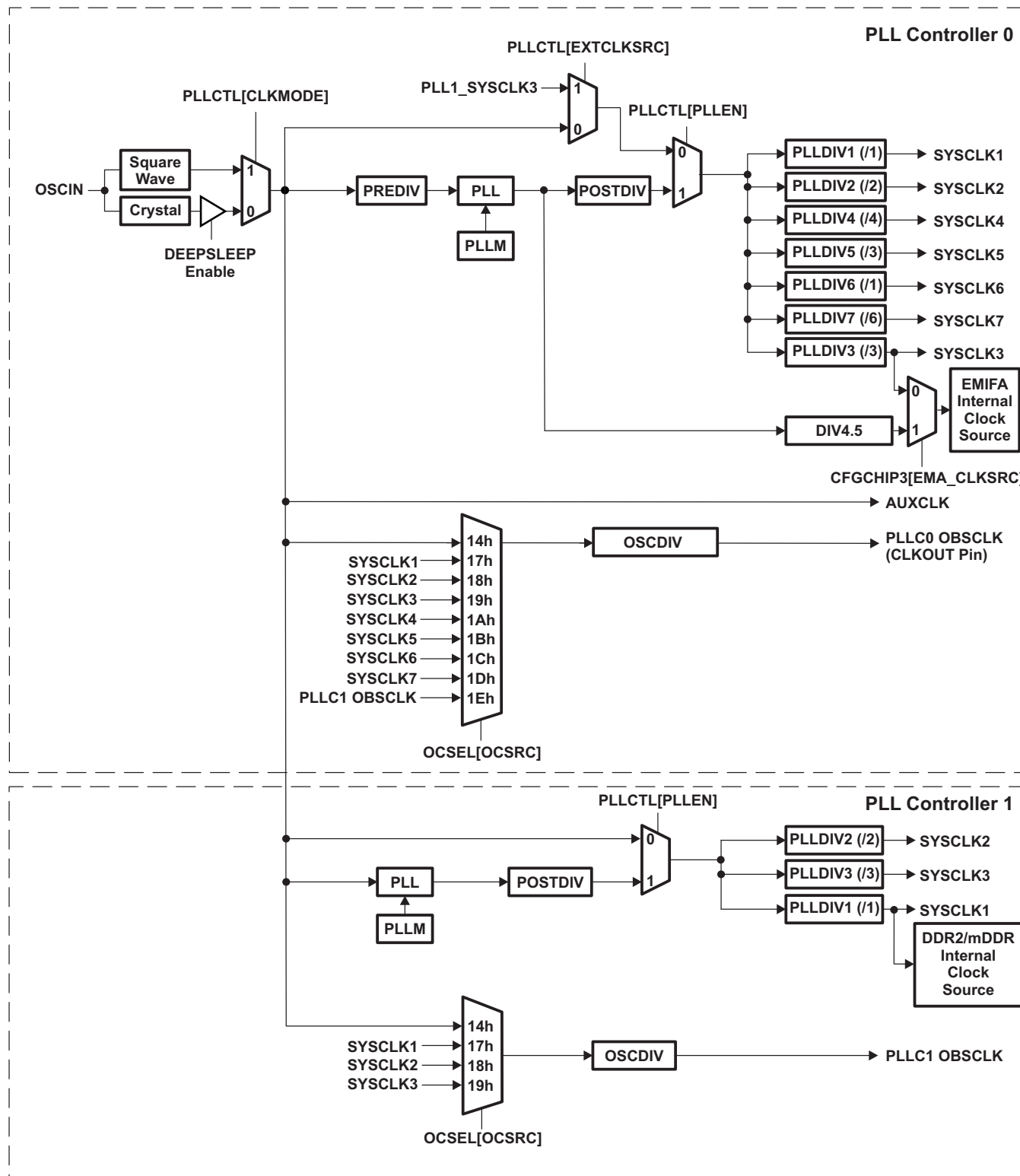
Figure 5-9. PLL Topology
