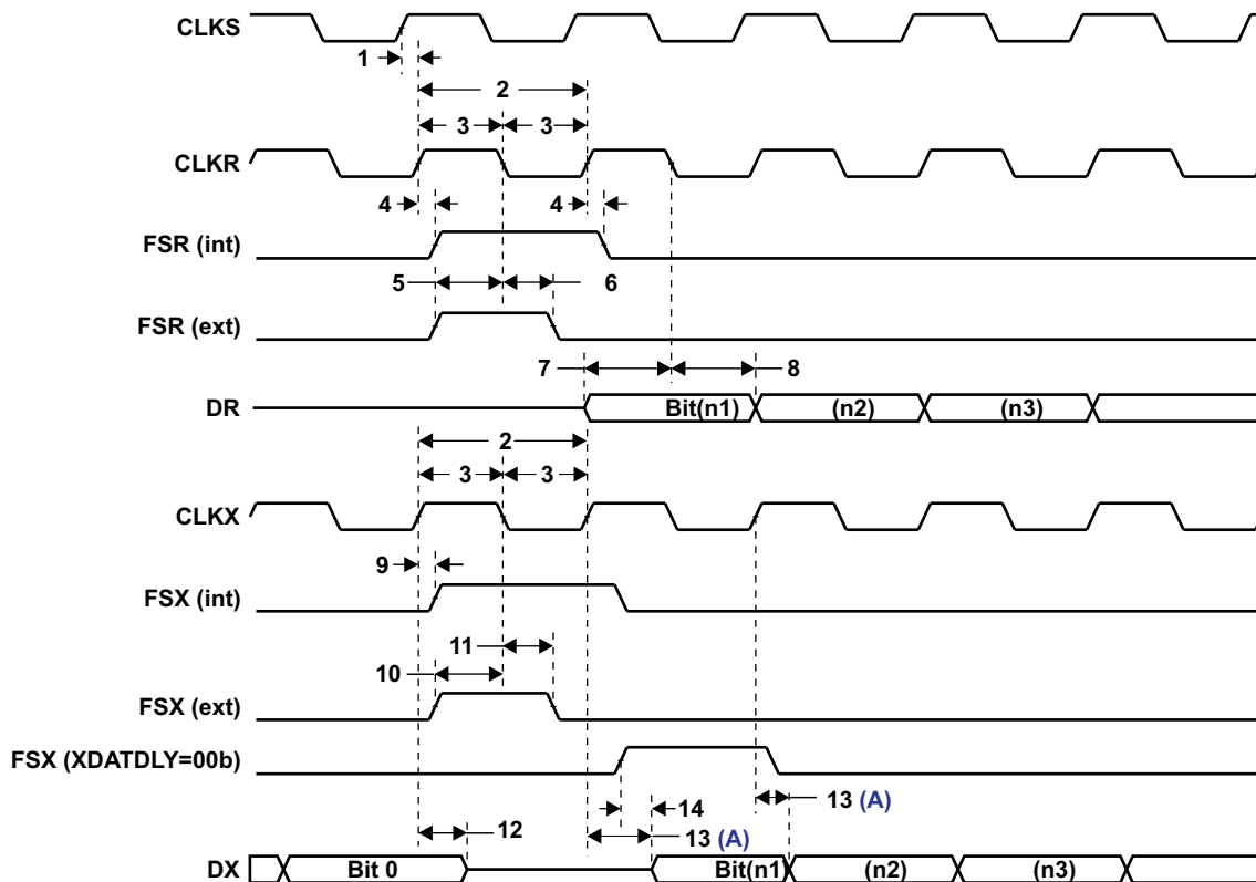
Figure 5-32. McBSP Timing
